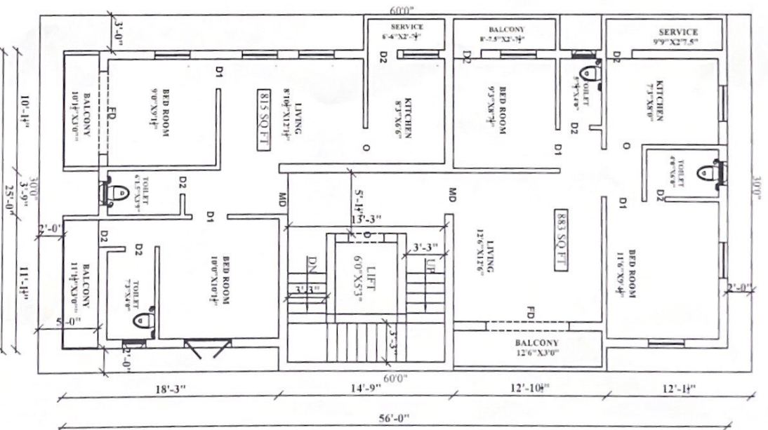
FIRST, SECOND & THIRD FLOOR PLAN
